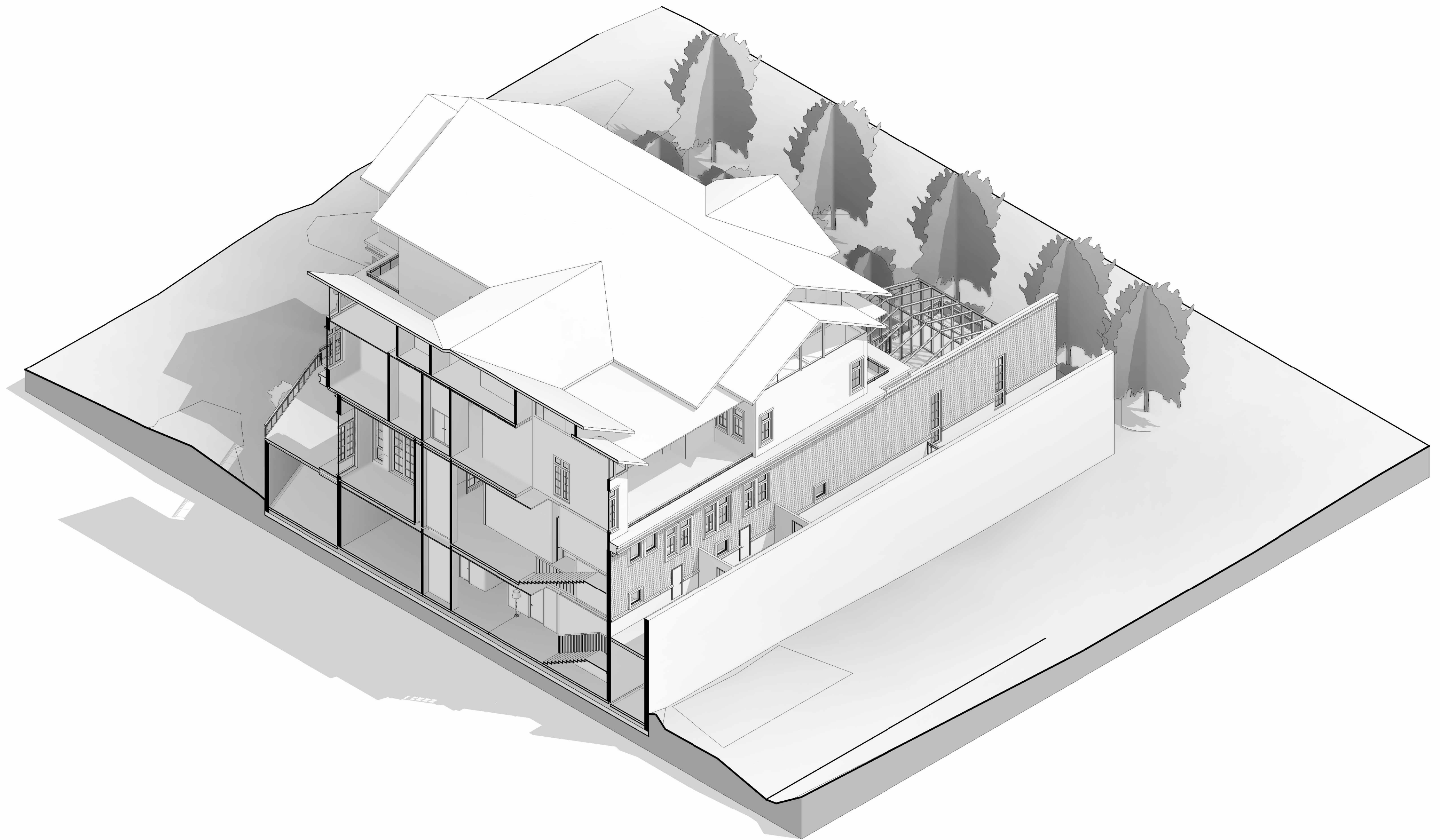
1 3D Section AA
